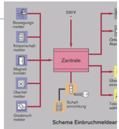
Schematic of a burglar alarm system
